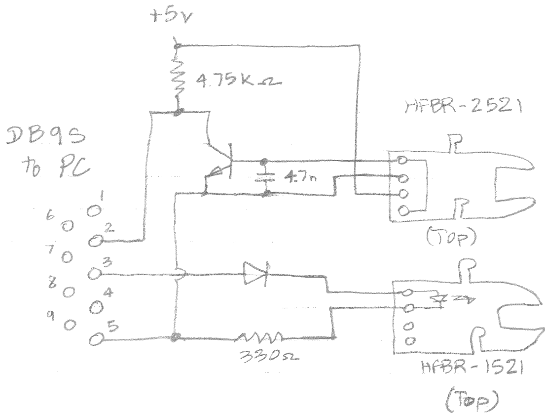
RS-232 / fiber Optic Converter
